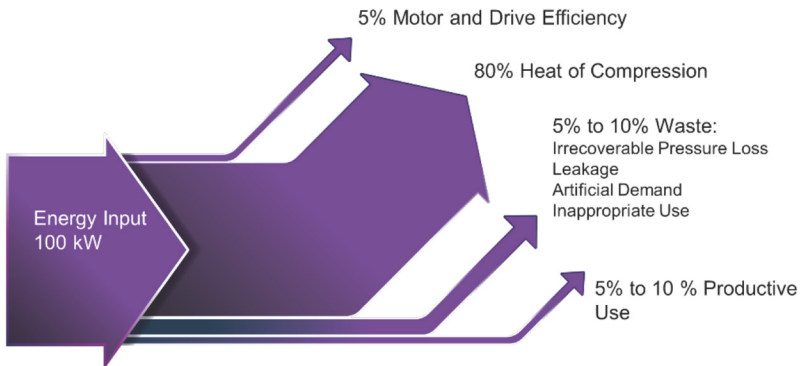
Figure 1. Typical Compressed Air Power Sankey
