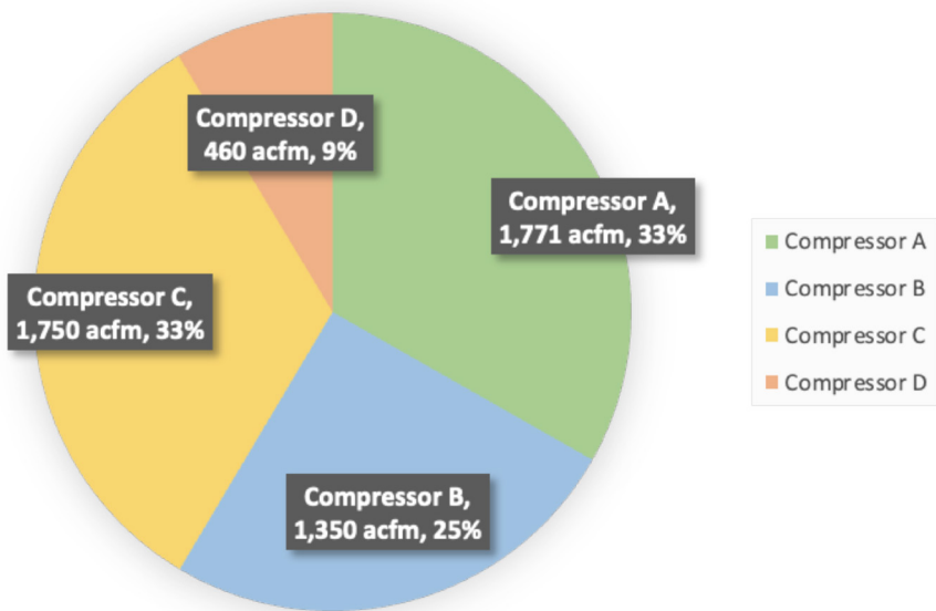
Figure 7. Summary of Airflow Capacity by Compressor
