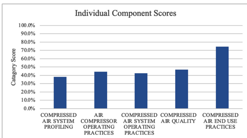
Figure 8. Summary of Compressed Air Scoping Tool Results.
